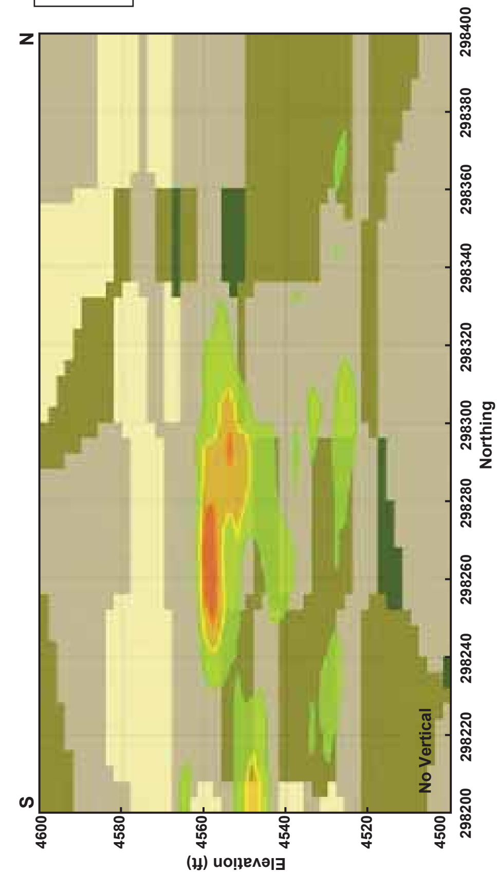
Figure 5-20. North-south vertical cross-section through the combined TCE/soil model at an easting of 1,856,110 ft.
